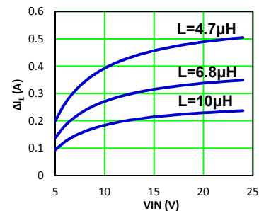
V_{\text{OUT}}=3.3\text{V} , F_{\text{OSC}}=1.2\text{MHz}
