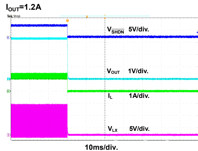
Figure 15. Power Off through \overline{SHDN} Waveform
