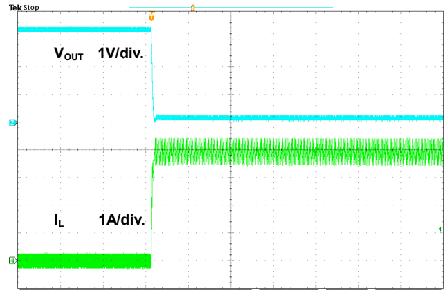
200µs/div. Figure 17. Short Circuit Test
