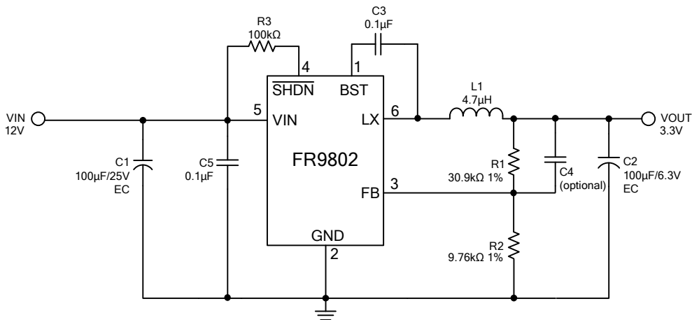
Figure 3. C_{IN}/C_{OUT} use Electrolytic Capacitors Application Circuit
