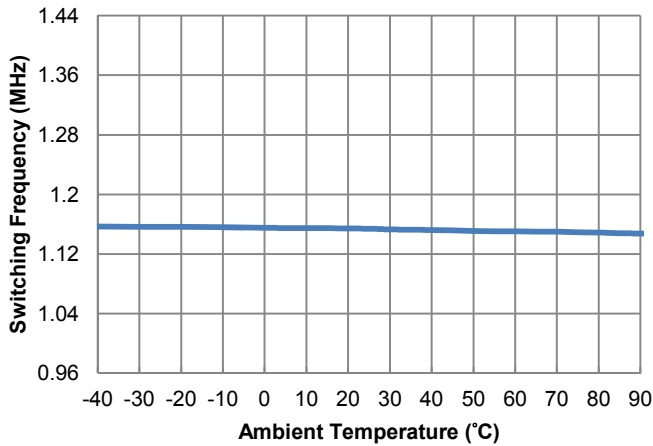
Figure 9. Switching Frequency vs. Temperature
