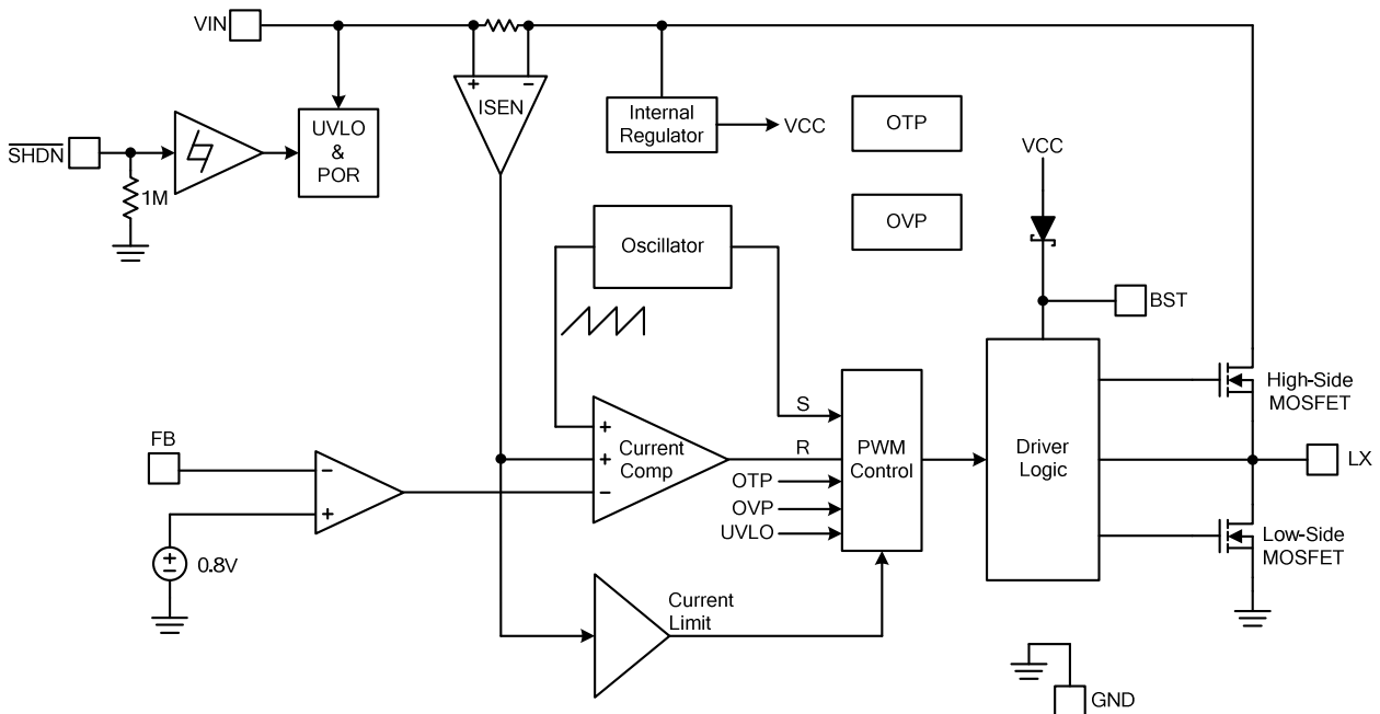
Figure 4. Block Diagram of FR9802
