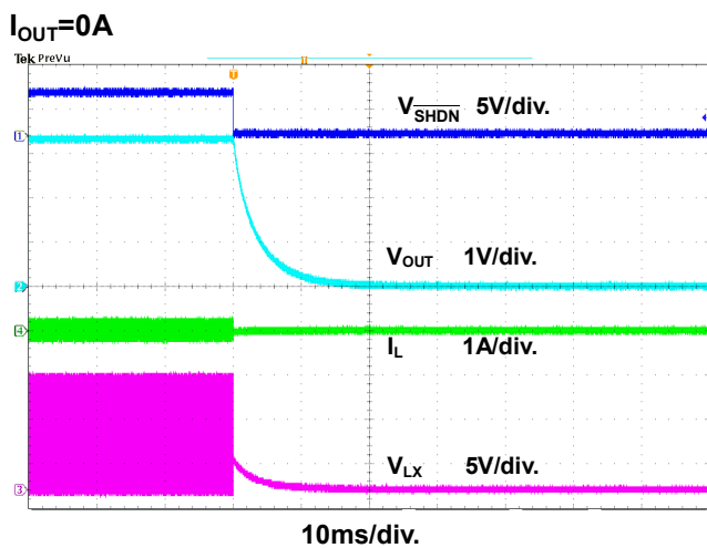
Figure 14. Power Off through \overline{SHDN} Waveform
