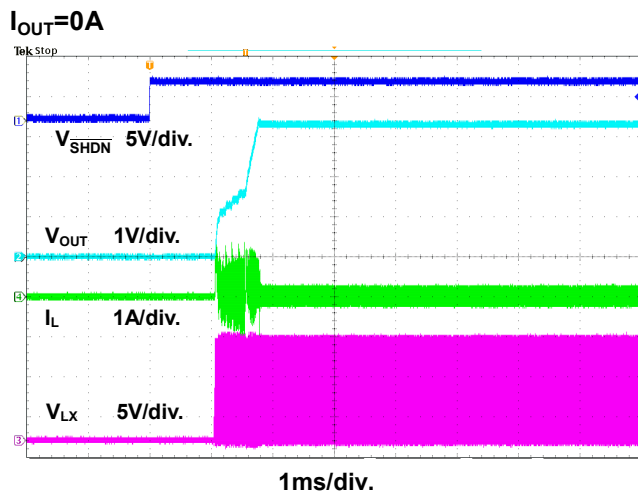
Figure 12. Power On through \overline{SHDN} Waveform
