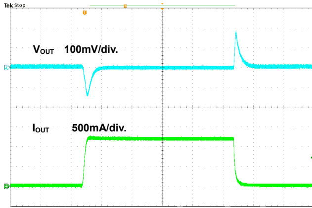
200µs/div. Figure 16. Load Transient Waveform
