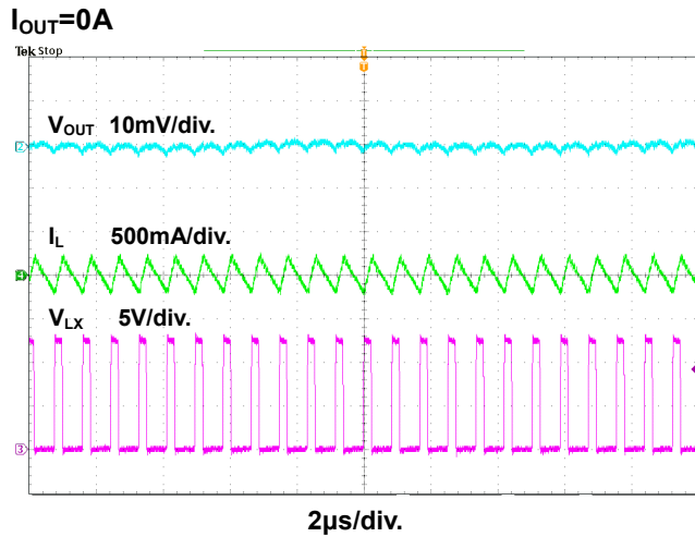
Figure 10. Steady State Waveform
