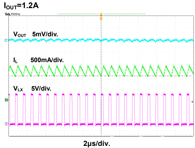
Figure 11. Steady State Waveform
