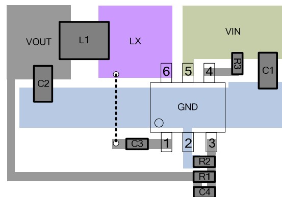
Figure 18. Recommended Layout Diagram
