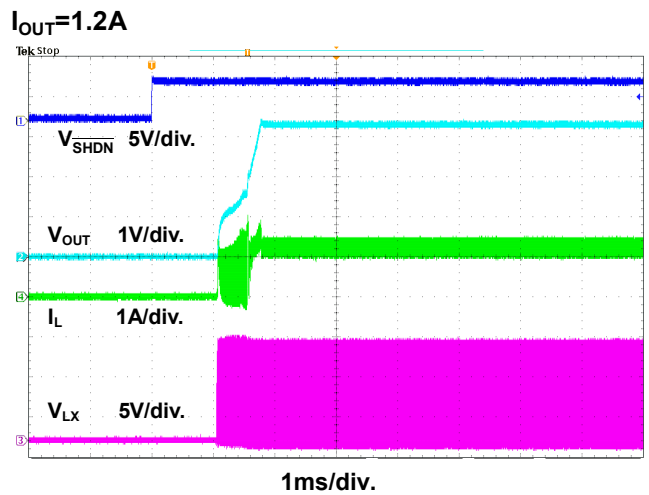
Figure 13. Power On through \overline{SHDN} Waveform
