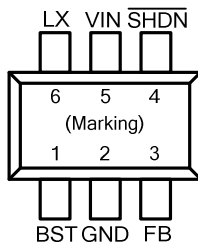
Figure 1. Pin Assignment of FR9802
